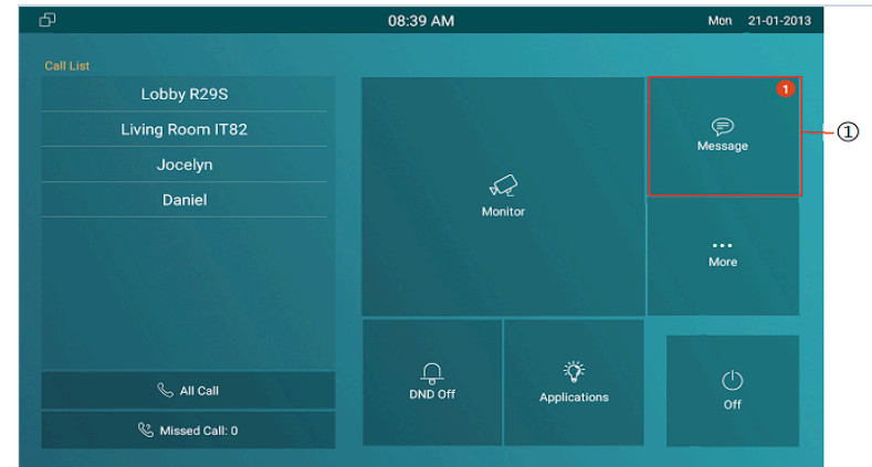
Figure 2.5 -1 Message
