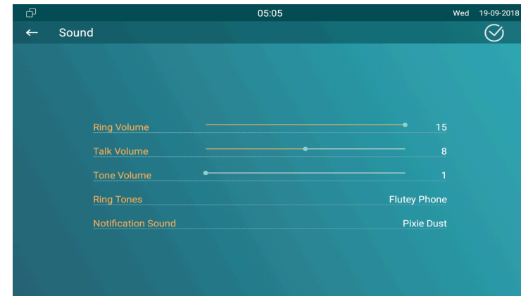
Figure 3.4.5-1 Sound setting
