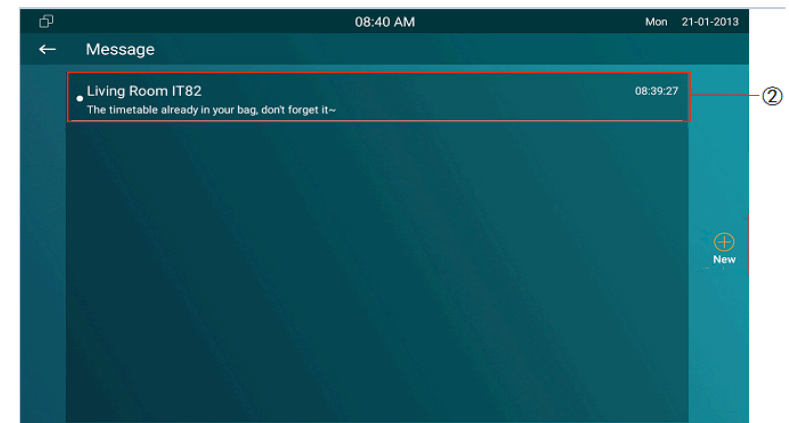
Figure 2.5.1-1 Text message
