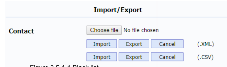
Figure 3.5.4-1 Black list
